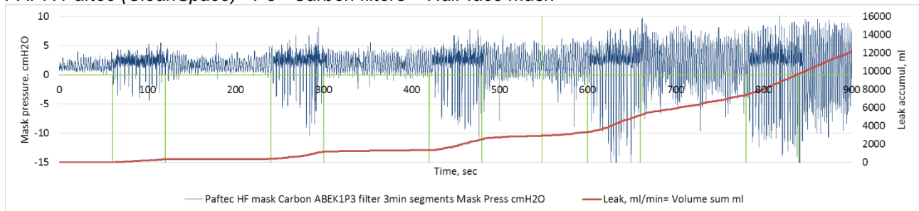
PAPR Paftec (CleanSpace) +P3+ Carbon filters + Half-face mask
