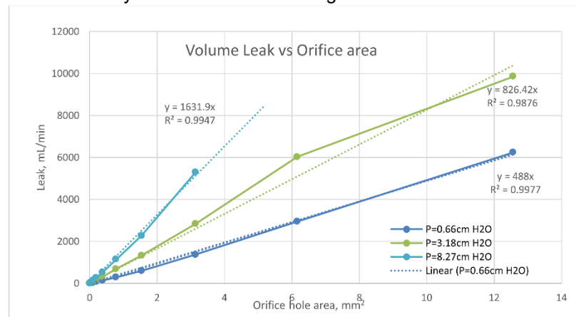
Figure 11: Leaks through the orifices expected to be linear with respect to opening area.
