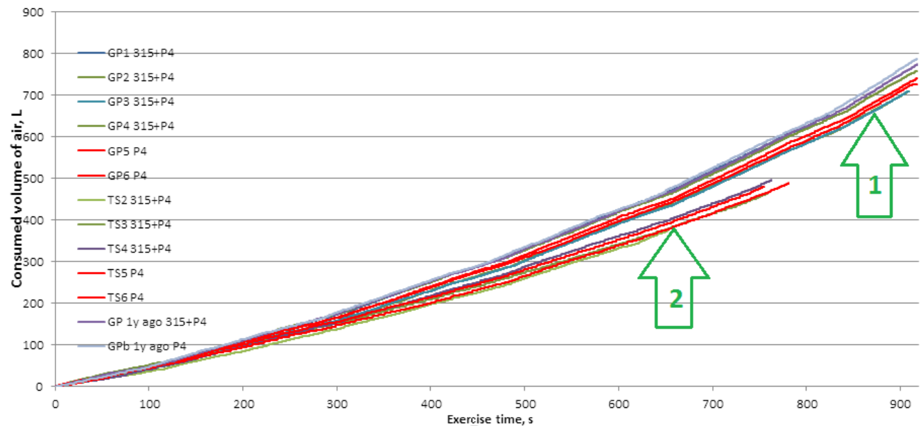
Figure 20: Air volume consumption for Subj 1 and Subj 2 at the same work profile for light resistance (red) and high resistance (dark) filters.
