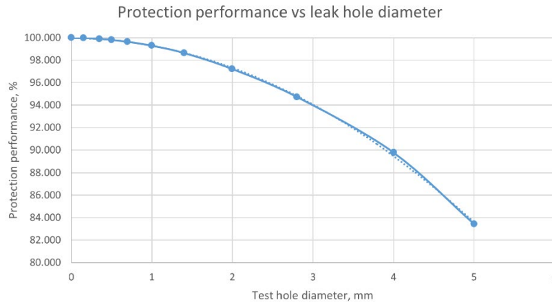
Figure 14: Graph representing the reduction in protection depending on the orifice diameter.
