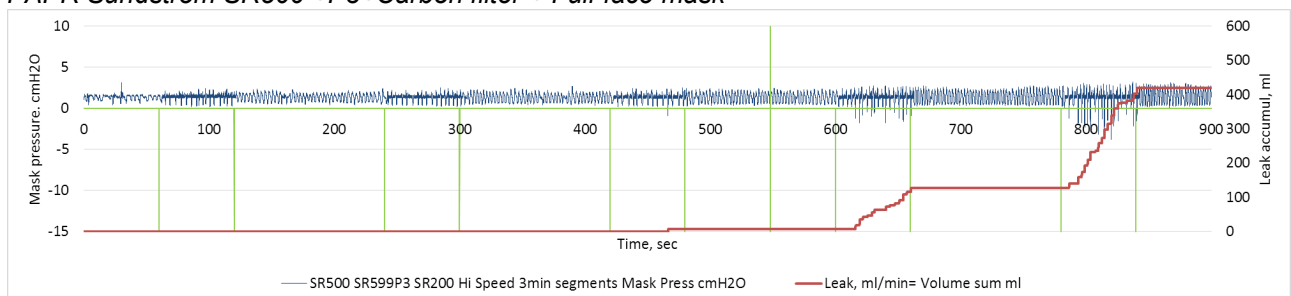
PAPR Sundström SR500 +P3+Carbon filter + Full-face mask
