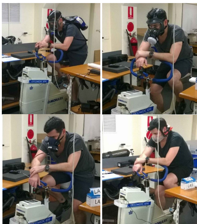
Figure 22: Test subject on the bicycle with different types of respirators.
