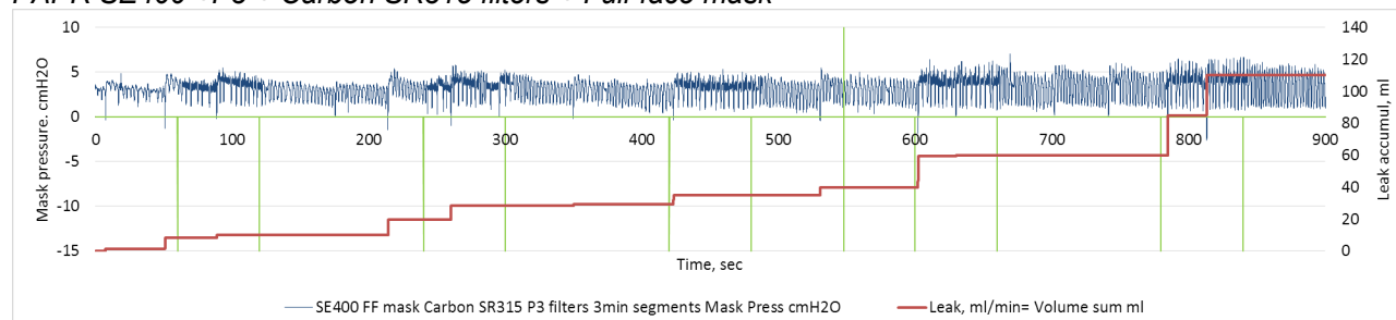
PAPR SE400 +P3 + Carbon SR315 filters + Full-face mask
