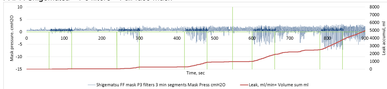
PAPR Shigematsu + P3 filters + Full-face mask
