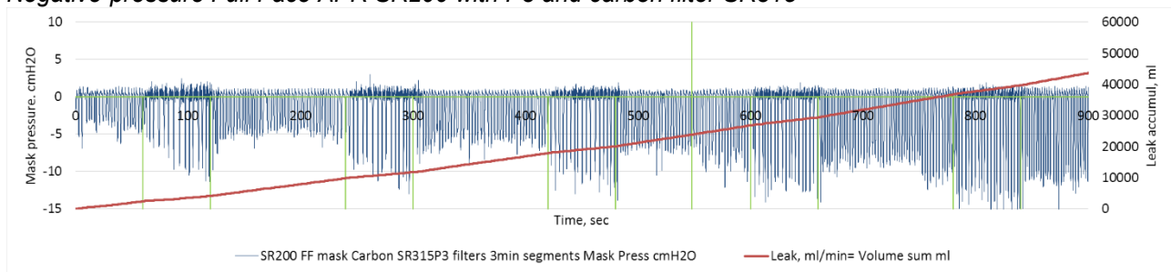
Negative-pressure Full Face APR SR200 with P3 and carbon filter SR315
