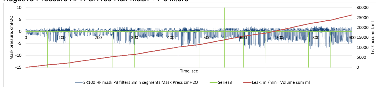
Figure 24 SR100 negative pressure Half mask + P3 filters.
