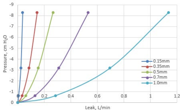
Figure 13: Pressure vs leak flow for orifices up to 1 mm diameter only.
