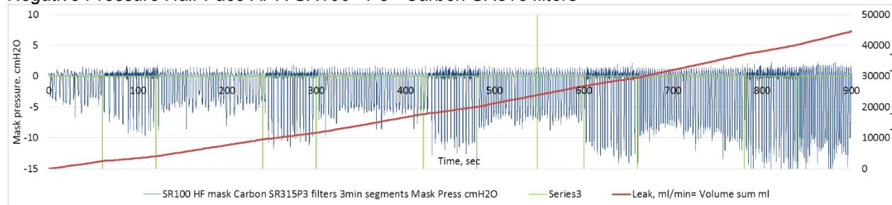
Negative Pressure Half-Face APR SR100 +P3+ Carbon SR315 filters
