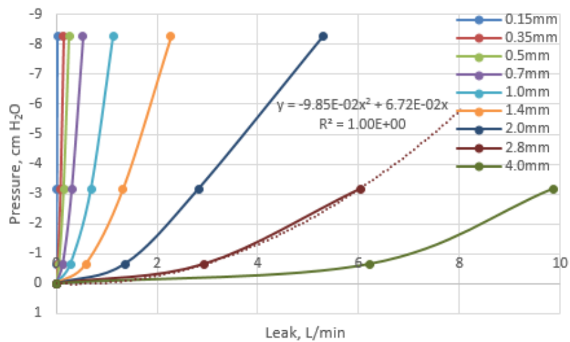
Figure 12: Pressure vs leak flow for all orifices.
