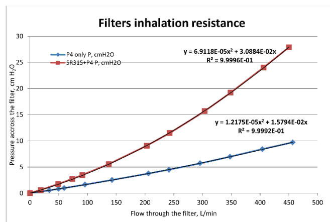
Figure 19: Low and high breathing resistance filters pressure-flow characteristics.
