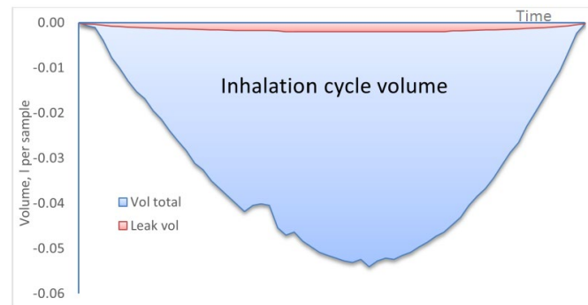
Figure 17: Inhalation Volume through the filter and through the orifice.
