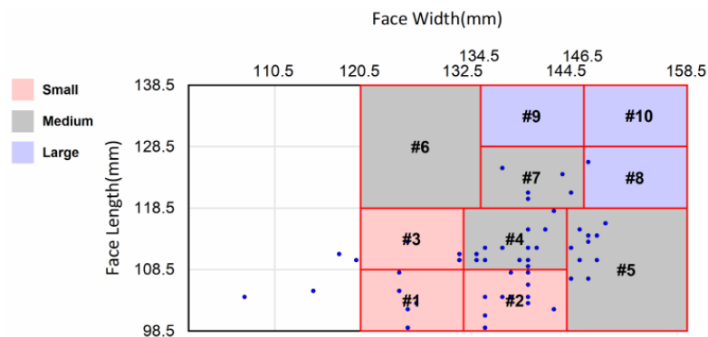
Figure 3. Distribution of study participants in the NIOSH bivariate fit test panel.
