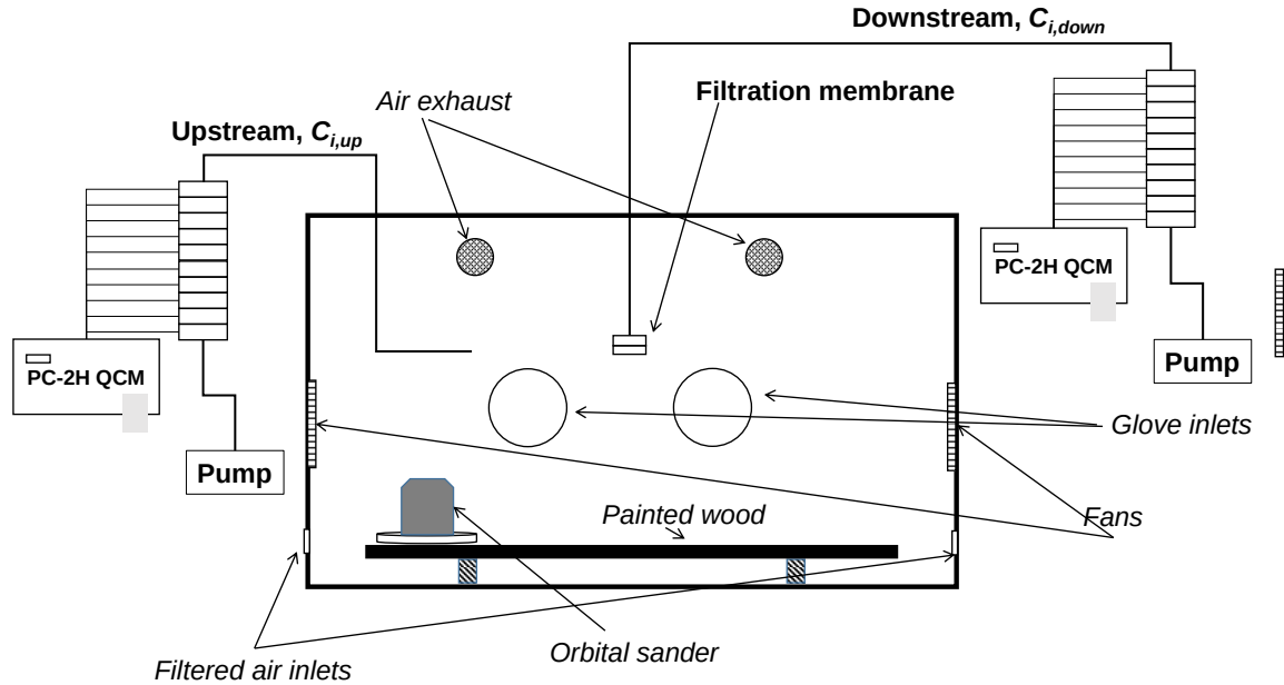
Figure 1. Schematic diagram of the experimental apparatus. Paint dust is generated into the chamber. The generated aerosol is measured in the chamber (Upstream, C_{i,up} ) and after the filtration membrane (Downstream, C_{i,down} ).
