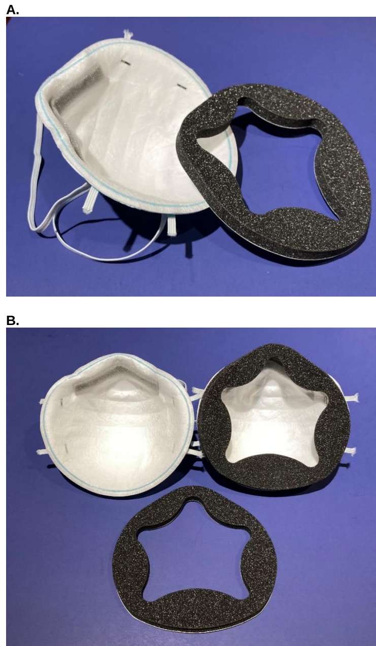
Figure 1. Faceseal prototype: FFR assembly (A); Unmodified and Faceseal-equipped N95 FFRs side-by-side along with a ready-to-be-sealed \frac{1}{4} -inch thick thermoplastic copolymer element (B).
