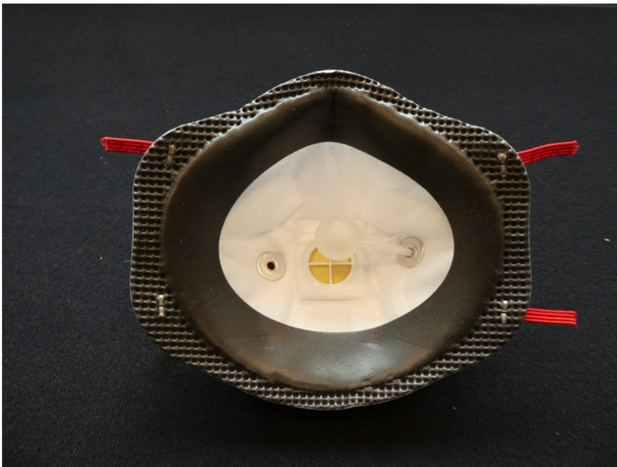
Figure 2. Example FFP3 mask with metal sampling ports in place.
