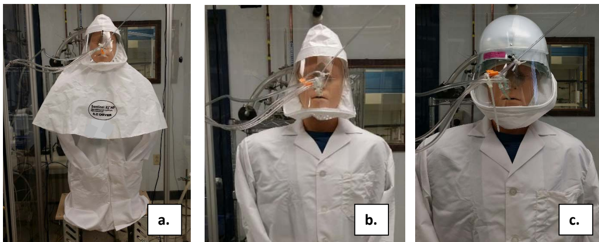
Figure 1. PAPR Models.
