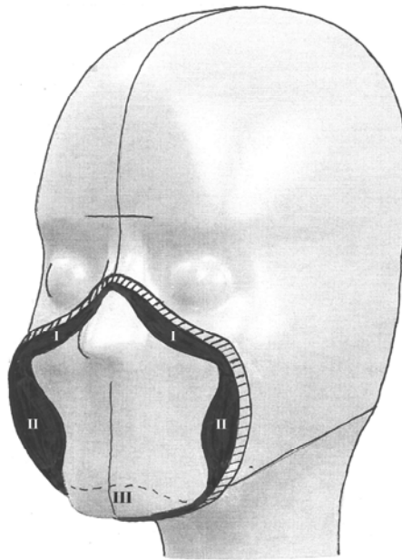
Figure 3. The new face seal on the human face.
