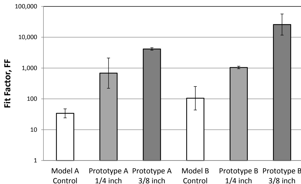
Figure 4. Fit Factor averaged over three donnings (one subject) for two control and four prototype respirators (with heating).
