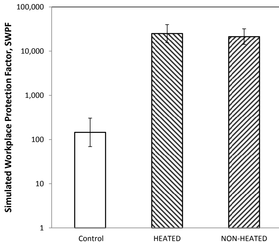
Figure 5. Simulated Workplace Protection Factor averaged over nine tests (three donnings on each of the three subjects) for the control and new respirator with and without heating. Evaluation in the operating room during electrocautery-based surgical procedure.
