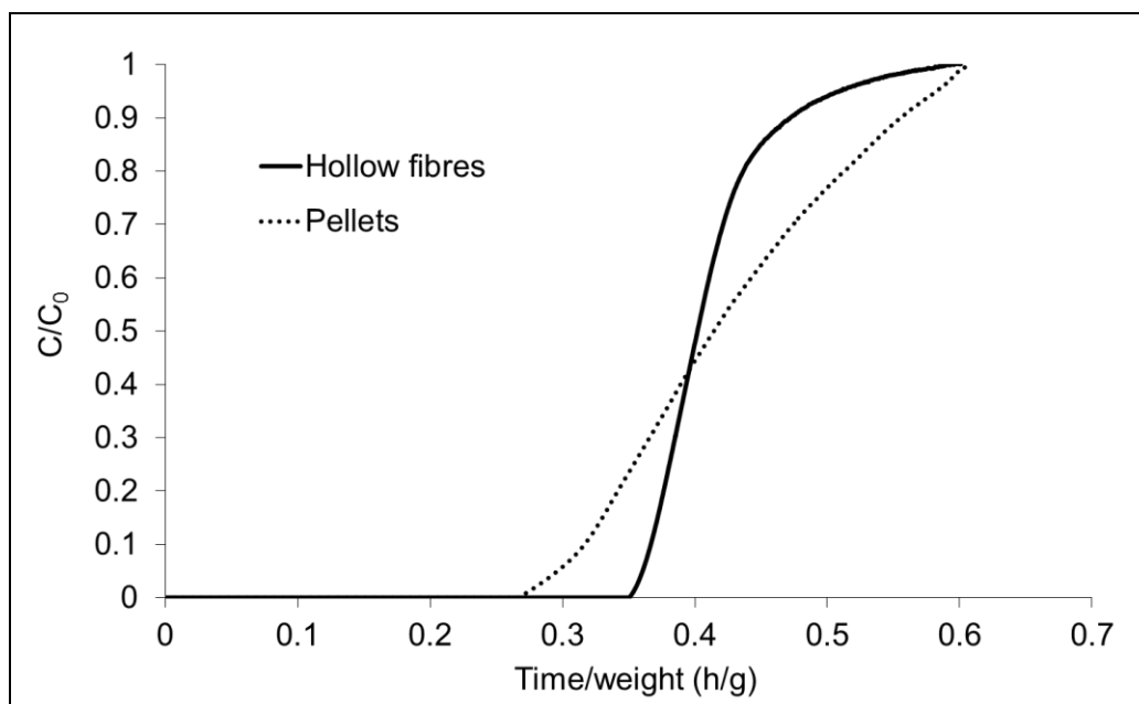
Figure 6. Experimental breakthrough curves per weight (hours/gram) for 5 cm long x 2 cm diameter hollow fibre (solid line) and packed bed (dotted line) modules challenged with 800 ppm 1 L/min \text{NH}_3 .
