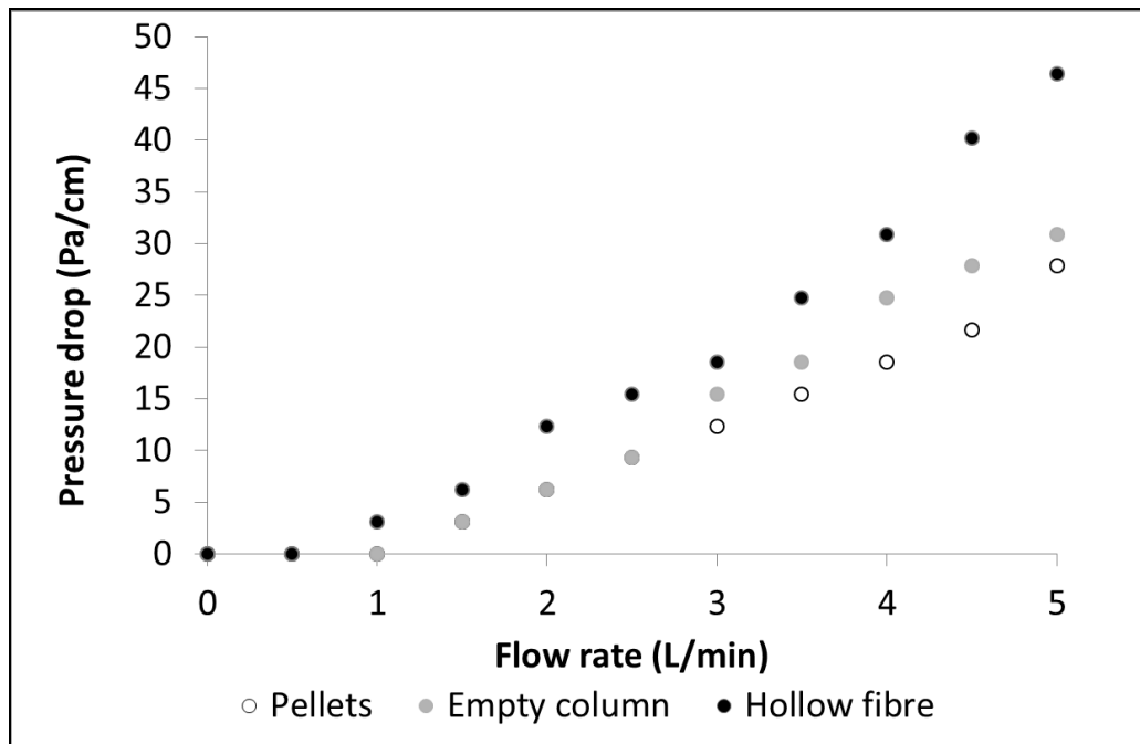
Figure 7. Pressure drop values measured from 5 cm long modules, calculated per cm bed depth for an empty module, a hollow fibre module and a 0.16 cm average particle diameter pellet module.
