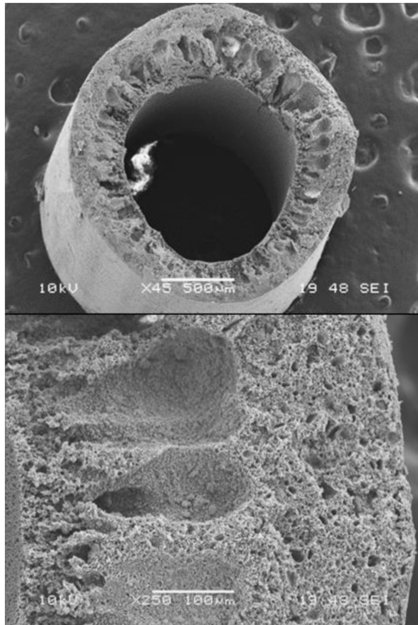
Figure 3. SEM images of hollow fibre containing AbScents 1000, x45 cross section (top) and x250 cross section (bottom).
