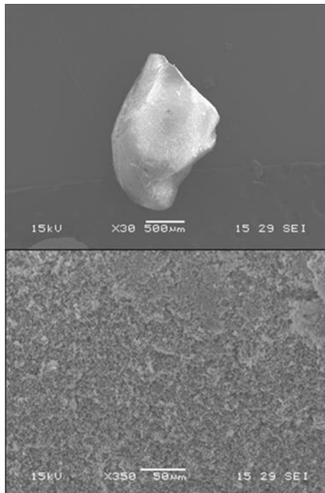
Figure 2. Scanning electron microscope (SEM) images of the surface of a AbScents 1000 adsorbent pellet, x30 (top) and x350 (bottom).
