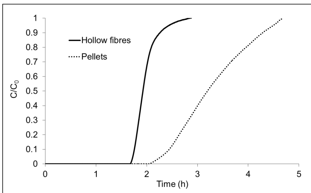
Figure 5. Experimental breakthrough curves for 5 cm long x 2 cm diameter hollow fibre (solid line) and packed bed (dotted line) modules challenged with 800 ppm 1 L/min \text{NH}_3 .
