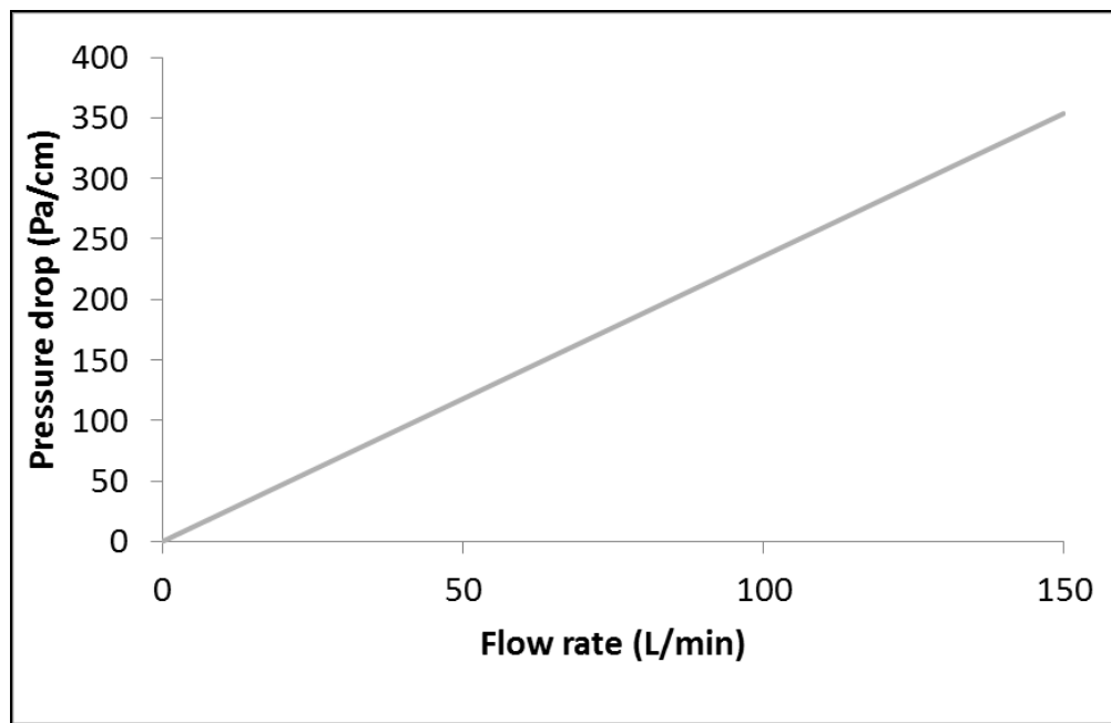
Figure 8. Extrapolated pressure drop/cm for 5 cm long x 2 cm diameter hollow fibre modules using the Hagen-Poiseuille equation.
