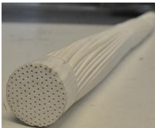
Figure 1. An example of a hollow fibre module.
