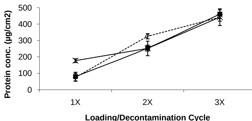
Figure 2. Average protein concentrations ( \mu\text{g}/\text{cm}^2 ) on FFR coupons loaded with HSL droplet nuclei for successive cycles of loading without decontamination (◇), with steam (×), and UVGI (■).
