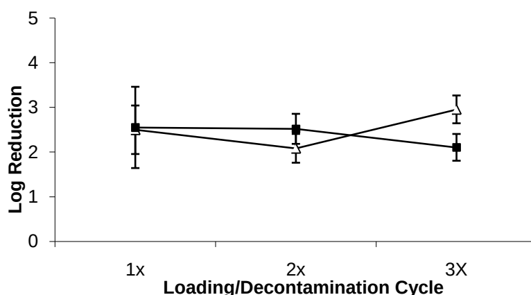
Figure 3. The log reduction of MS2 for successive loading/steam decontamination cycles. Droplet nuclei containing MS2 was generated from HSL (■) and LSL (▲) media.
