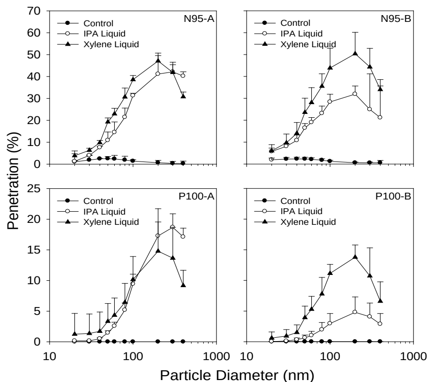
Figure 5: Penetrations of monodisperse NaCl (20–400 nm) particles for electret N95 (top row) and P100 (bottom row) FFRs from two manufacturers (A and B) at 85 L/min for 100% liquid IPA (open circles) and xylene (solid triangles). Error bar represents the 95% confidence interval (n = 3).
