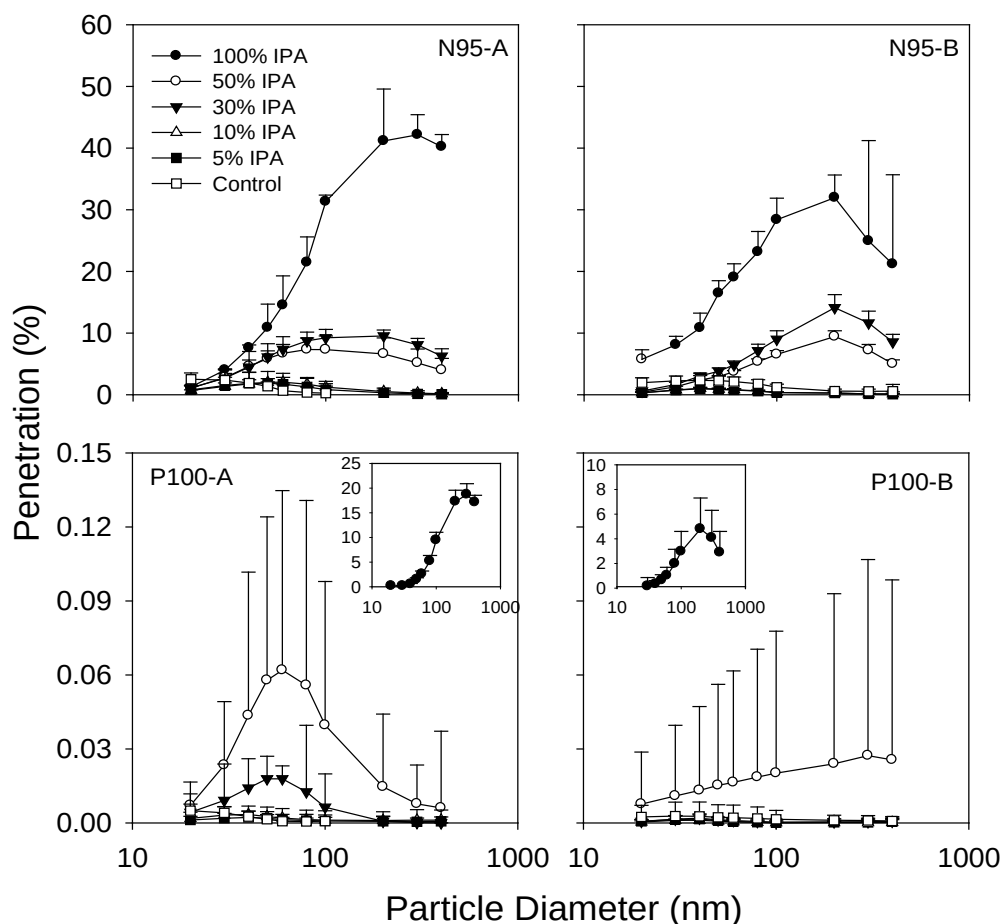
Figure 3: Penetration levels of monodisperse NaCl (20–400 nm) particles for electret N95 (top row) and P100 (bottom row) FFRs from two manufacturers (A and B) at 85 L/min for five concentrations of liquid IPA. Error bar represents the 95% confidence interval (n = 3). Insets in bottom row used to show penetration curves for 100% IPA treatment for the P100 FFR.
