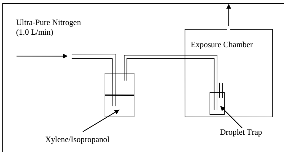
Figure 1. Isopropanol and xylene vapor exposure setup.
