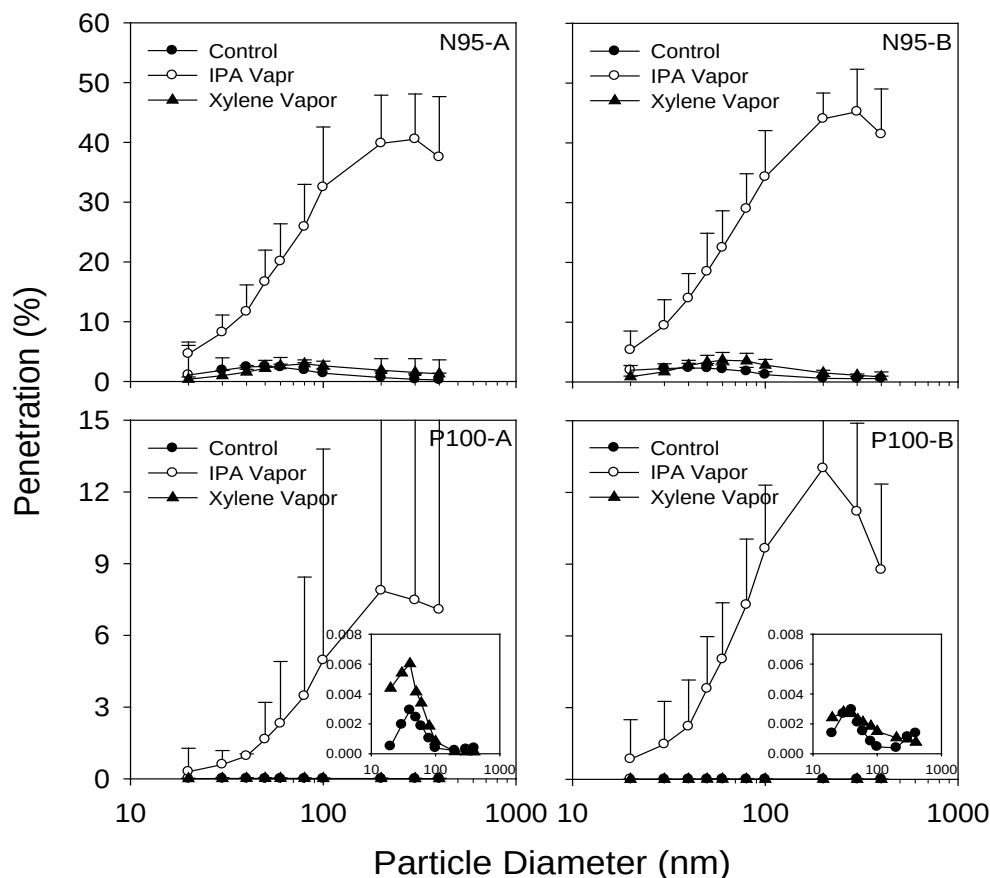
Figure 6: Penetrations of monodisperse NaCl (20–400 nm) particles through electret N95 (top row) and P100 (bottom row) FFRs from two manufacturers (A and B) at 85 L/min after 8 hour exposure to IPA (open circles) and xylene (solid triangles) vapors. Error bar represents the 95% confidence interval ( n = 3 ). Insets in bottom panels show penetration curves for control and 8 hour xylene exposure for the P100 FFRs.
