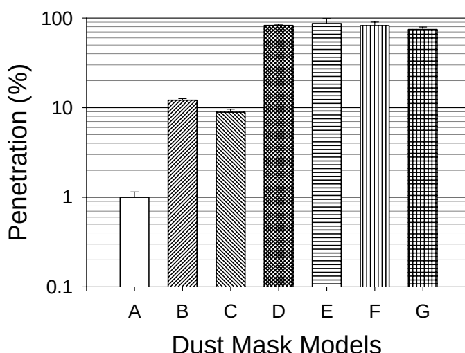
Figure 1. Penetration levels from the polydisperse aerosol test (PAT) method for the low (A)-, medium (B and C)-, and high (D, E, F, and G)-penetration category dust masks at 85 L/min flow rate.
