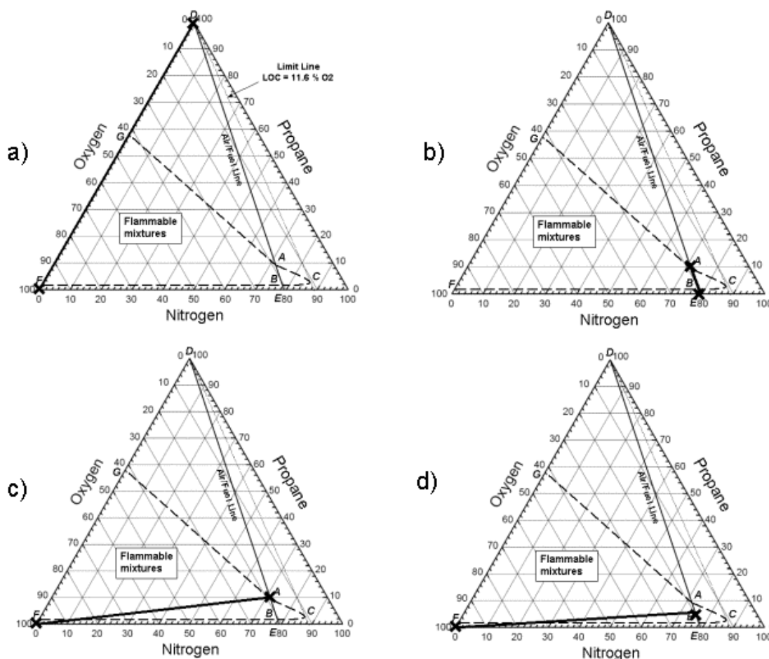
Figure 2. Flammability diagram for propane. Heavy line shows range of mixtures for a) leak of pure oxygen into pure propane, b) leak of air into 10% propane in air, c) leak of pure oxygen into 10% propane in air, and d) leak of pure oxygen into 5% propane in air.
