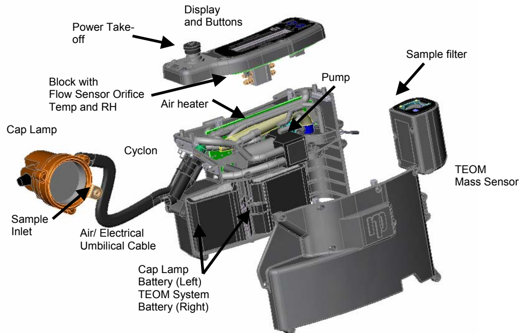
Figure 2. PDM internal components.
