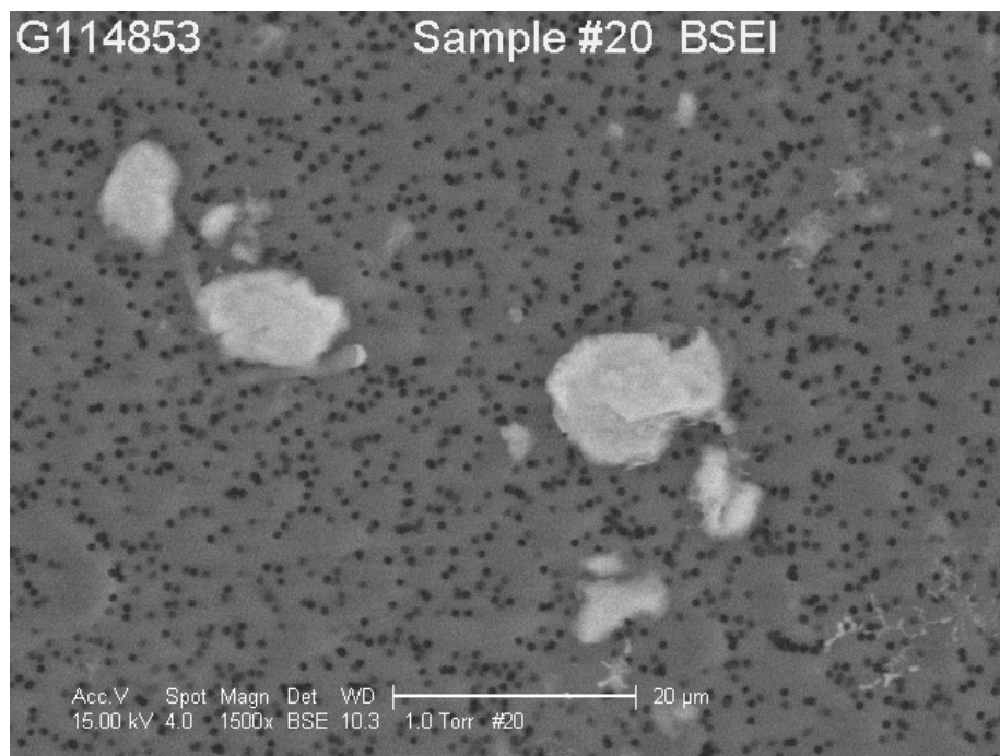
Figure 2. Photomicrograph of particles found on a C_i sample from one of the magnesium grinders. Magnesium was identified as a major component of the large particle in the right-center of the photo.
