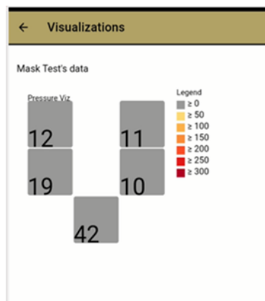
Figure 6. Heat Map with ADC Values in the Continuous Fit Monitoring System App
