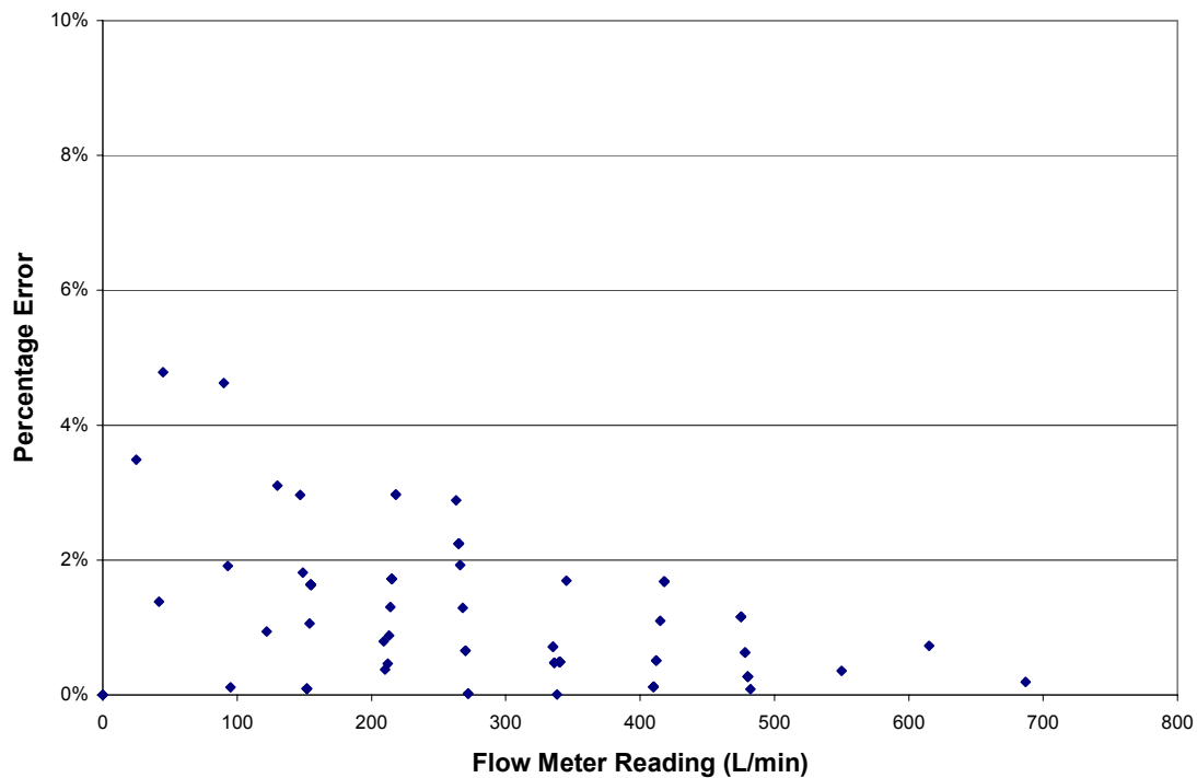
Figure 9. Flow meter errors as a function of flow meter reading.
