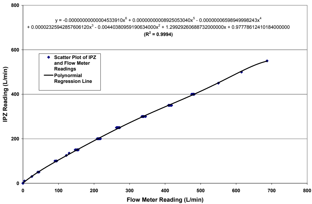
Figure 8. Plot of IPZ readings and data correction curve against flow meter readings.
