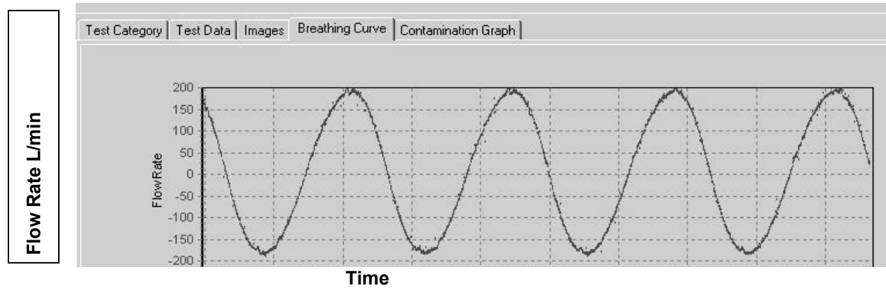
Figure 4. The flow rate from the IPZ breathing machine is shown as sine curve over time.
