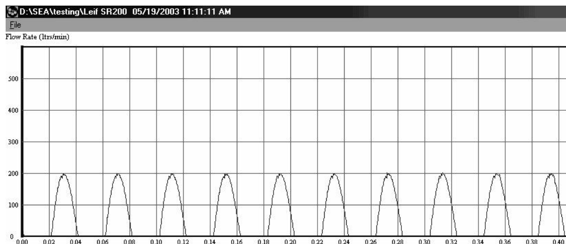
Figure 6. Flow rate (L/min) over time (The timeline is divided into 100ths of a minute. The graph shows 0.40 of a minute, or 24 seconds).
