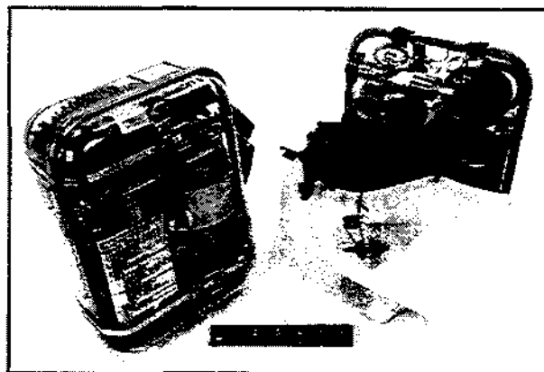
Figure 5. Cased and uncased Ocenco EBA 6.5 self-rescuer.
