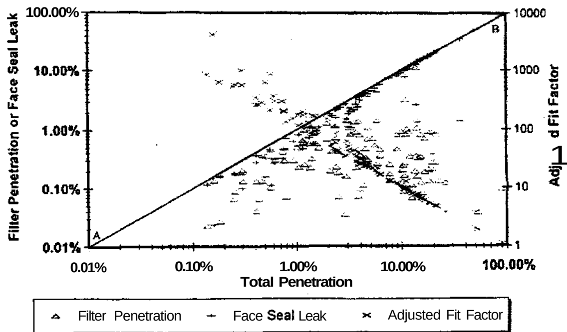
Figure 3. Scatter plot of filter penetration, face seal leak, and adjusted fit factor against total penetration.
