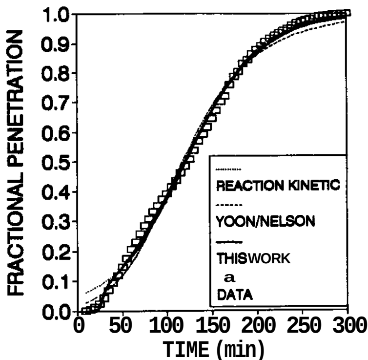
Figure 4. An unusually shaped breakthrough curve. 1000 ppm benzene, 90% RH preconditioned, 50% RH experimental, 53.3 L/min.
