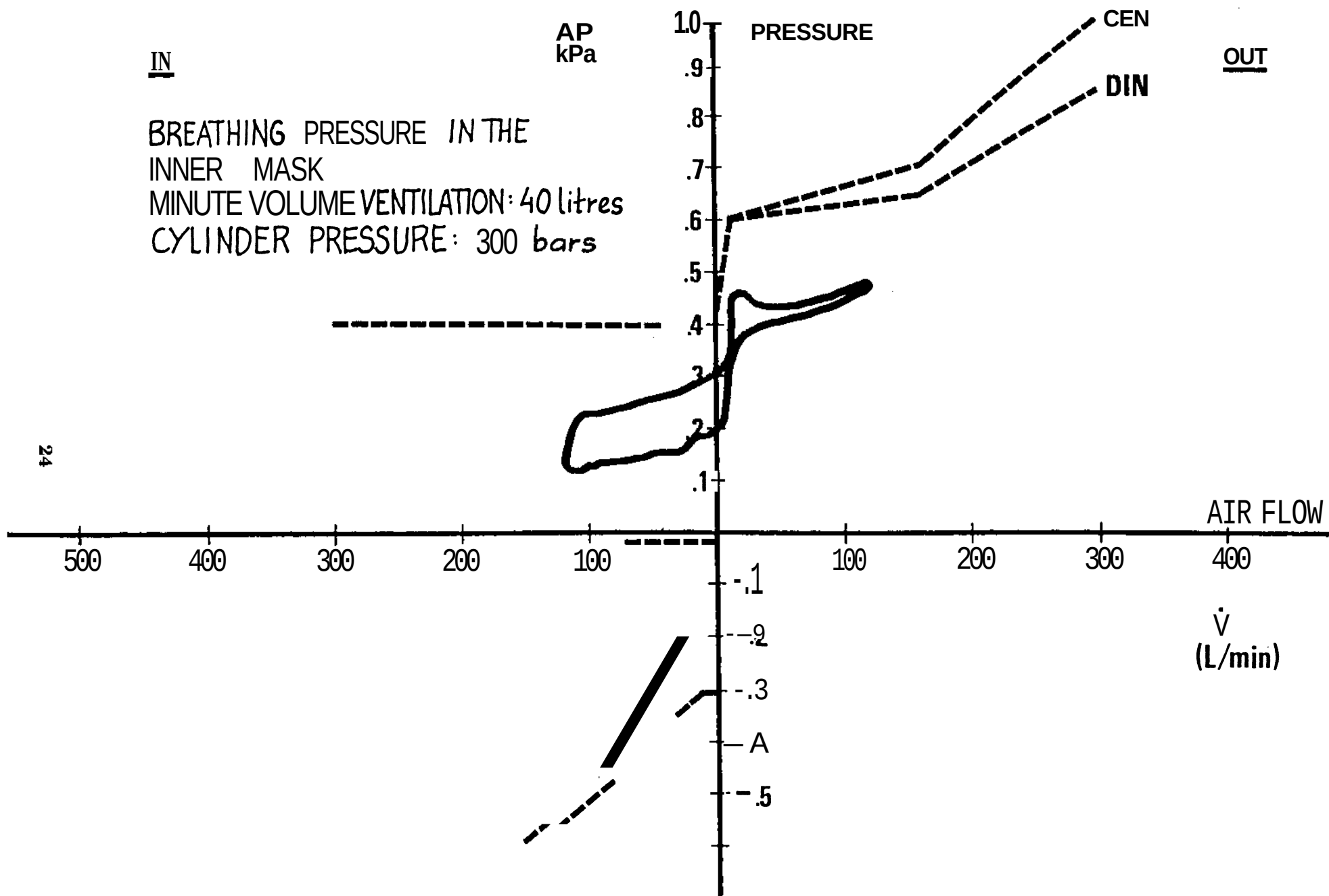
Figure 2. Pressure-volume diagram for open-circuit SCBA at moderate work rate and full gas supply.
