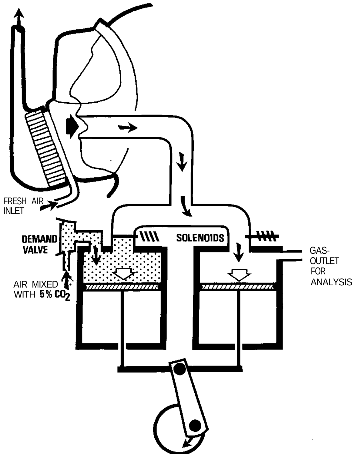
Figure 8. Test apparatus for measuring dead space.
