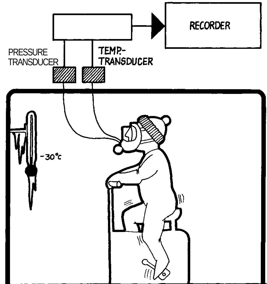
Figure 11. Human subject cold-test apparatus.
