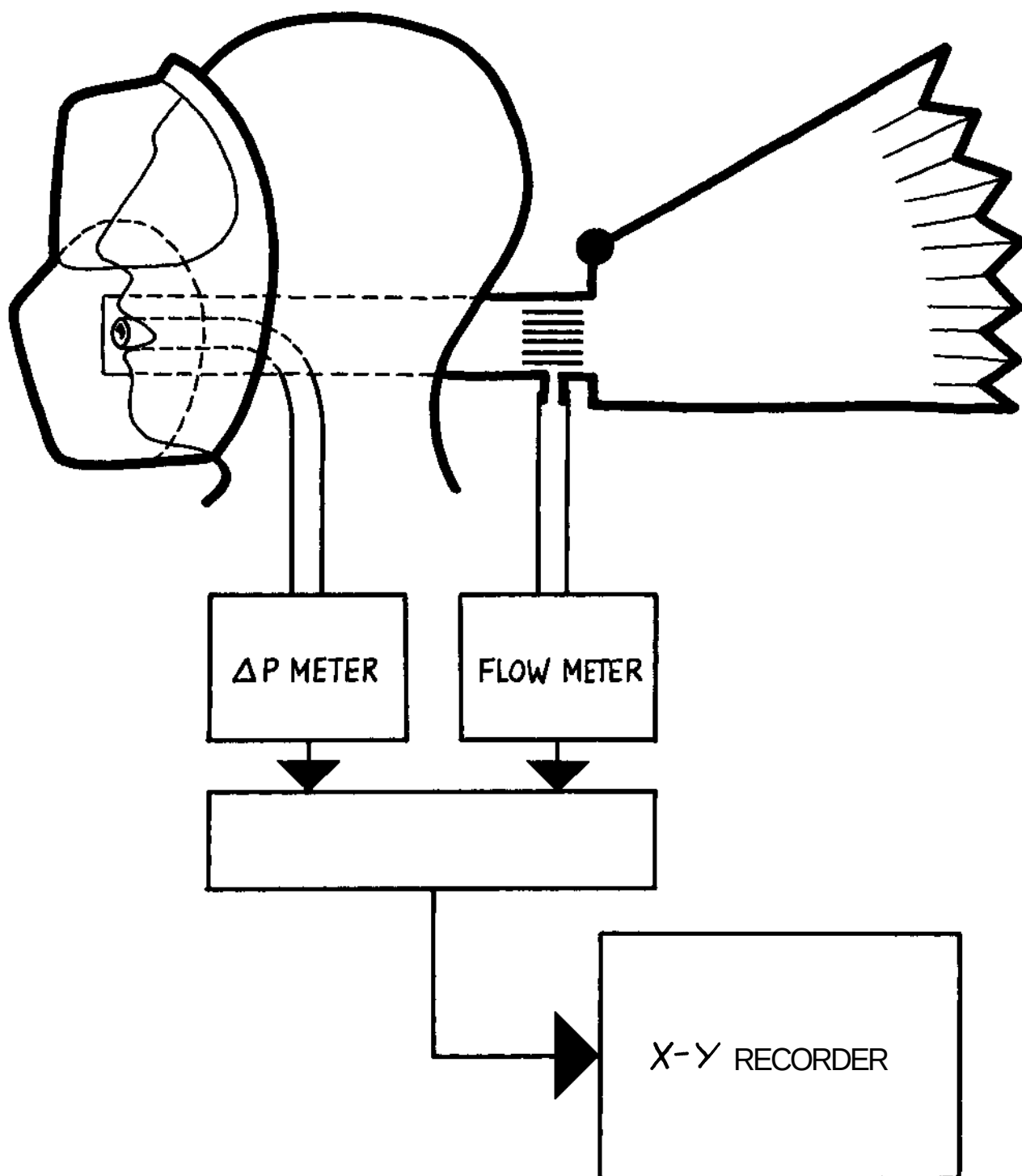
Figure 1. Suggested test program for firefighters' SCBA.
