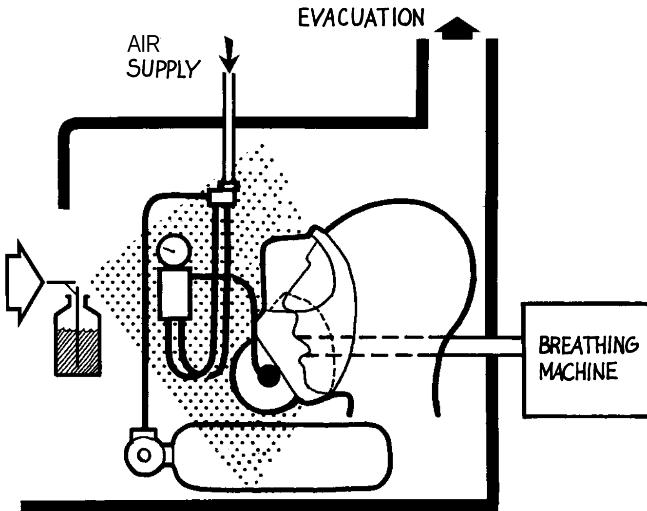
Figure 9. Apparatus for testing chemical exposure to SCBA.
