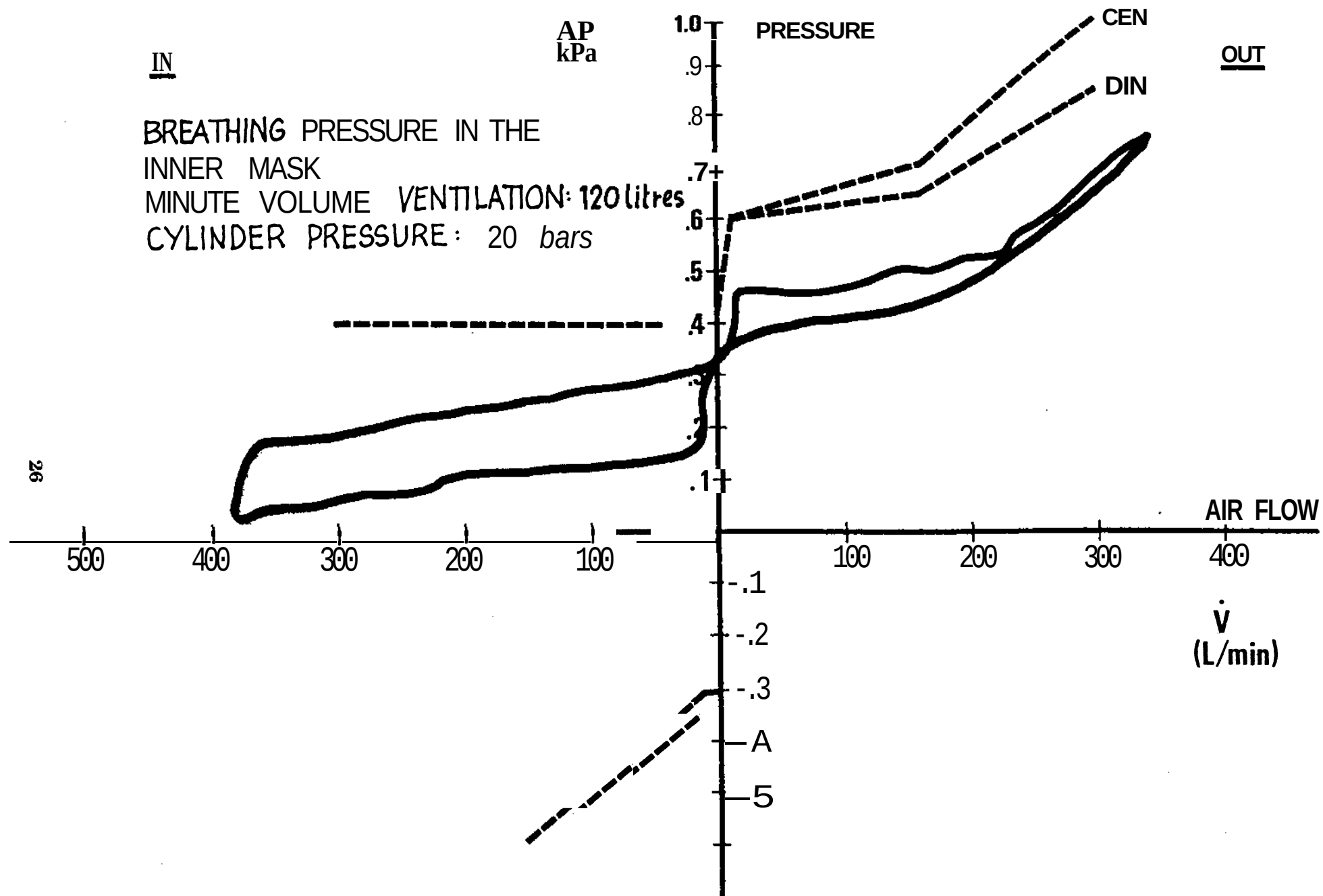
Figure 4. Pressure-volume diagram at high work rate and low gas supply.
