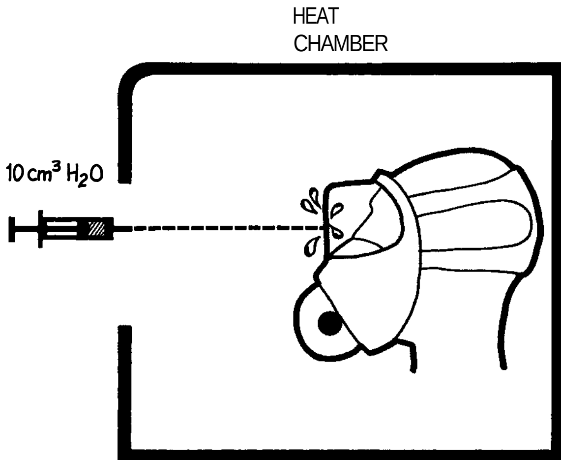
Figure 10. Heat and water test setup.
