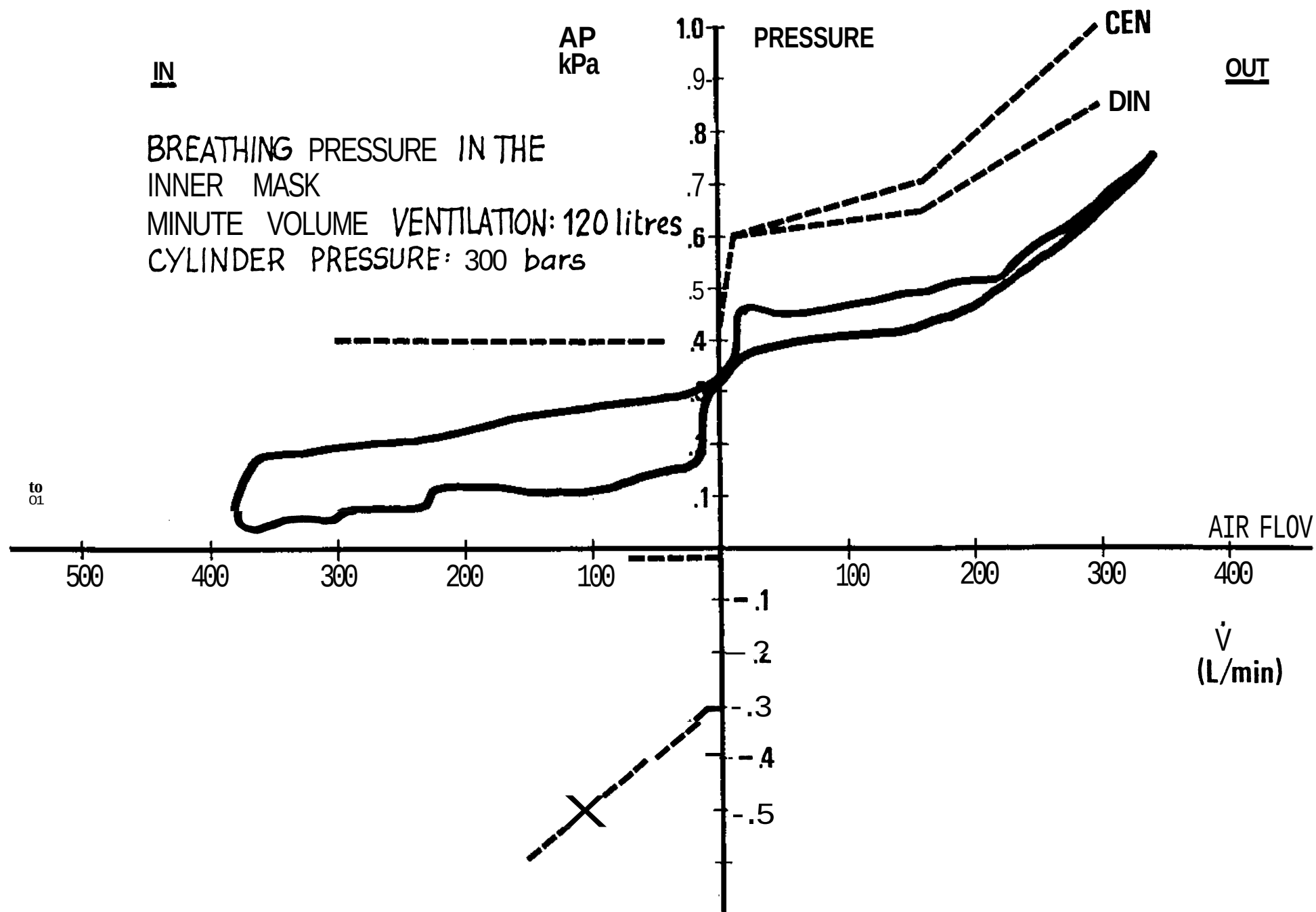
Figure 3. Pressure-volume diagram at high work rate and full gas supply.
