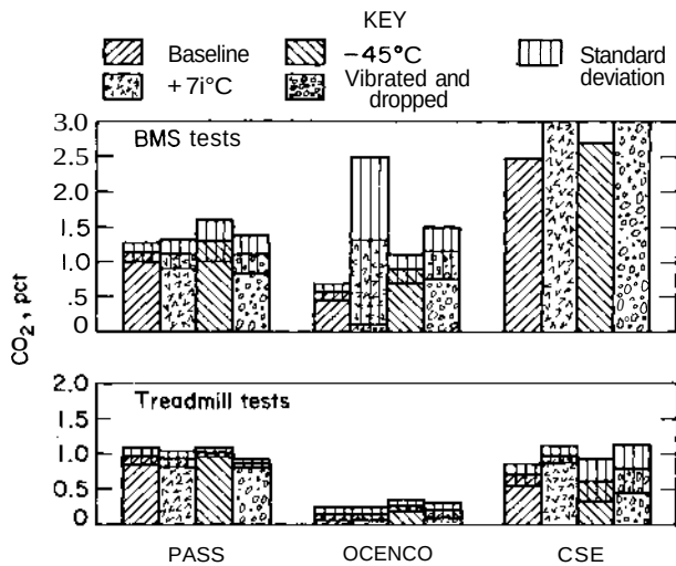
Figure 14. Average CO_2 concentration and standard deviation of 3 BMS and 3 treadmill tests for each environment and self-rescuer.
