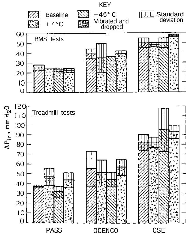
Figure 16. Average inhalation resistance and standard deviation of 3 BMS and 3 treadmill tests for each environment and self-rescuer.
