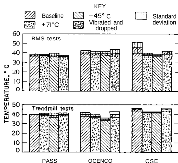
Figure 17. Average inhalation temperature and standard deviation of 3 BMS and 3 treadmill tests for each environment and self-rescuer.
