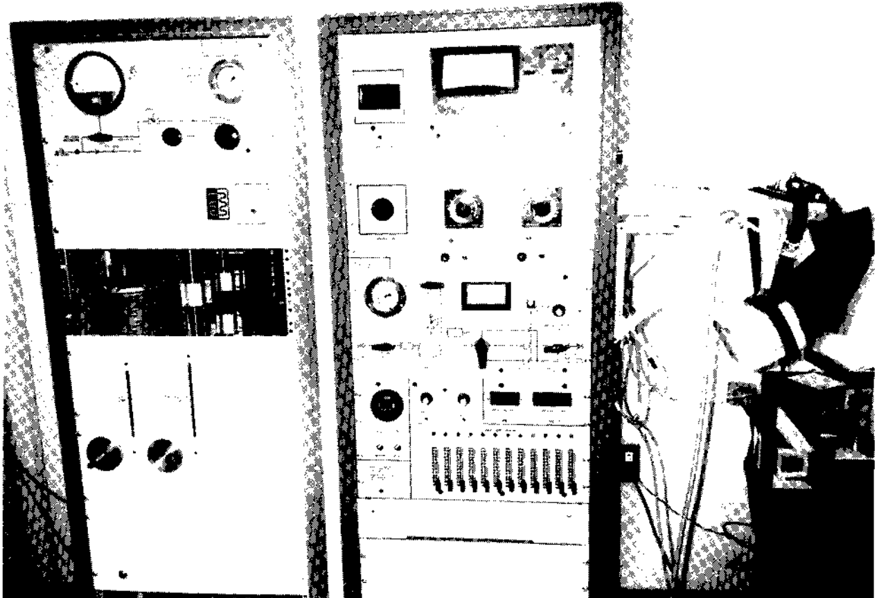
Figure 10. Breathing and metabolic simulator (BMS).
