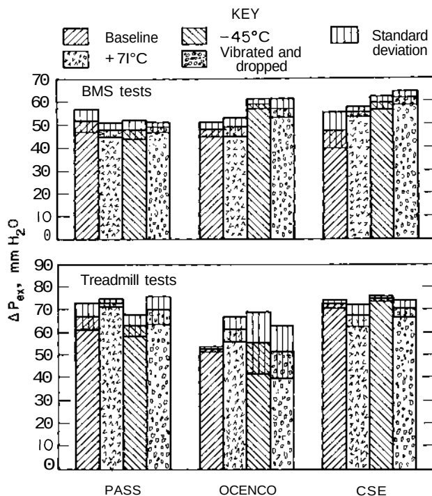
Figure 15. Average exhalation resistance and standard deviation of 3 BMS and 3 treadmill tests for each environment and self-rescuer.
