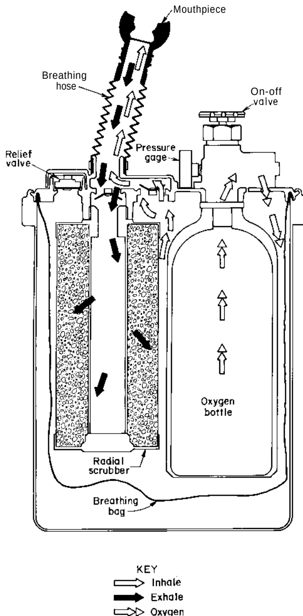
Figure 8. PASS 700 schematic.
