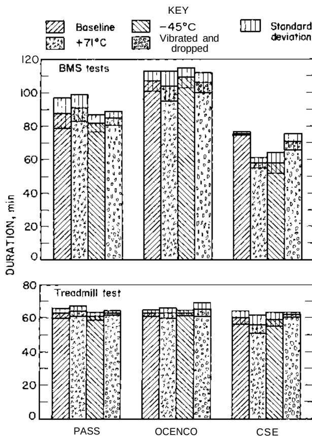
Figure 12. Average duration and standard deviation of 3 BMS and 3 treadmill tests for each environment and self-rescuer.
