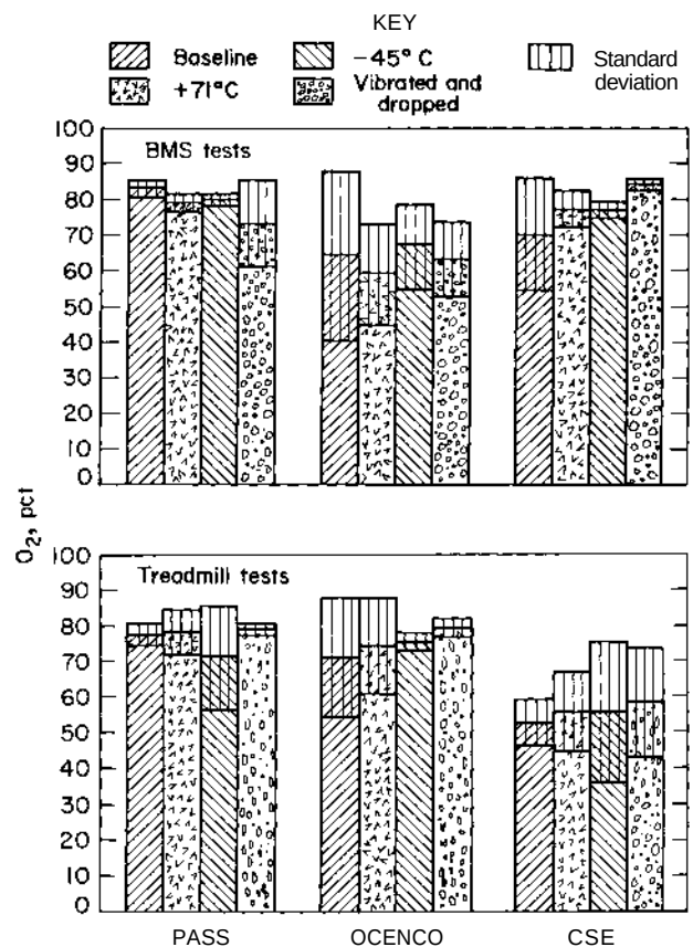
Figure 13. Average O 2 concentration and standard deviation of 3 BMS and 3 treadmill tests for each environment and self-rescuer.
