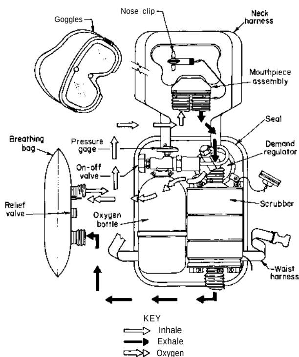
Figure 7. Ocenco EBA 6.5 schematic.
