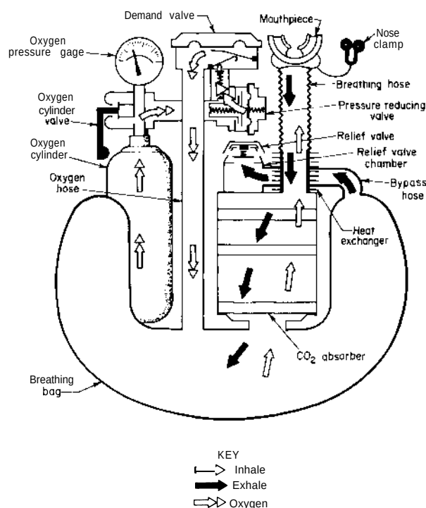
Figure 6. CSE AU-9A1 schematic.
