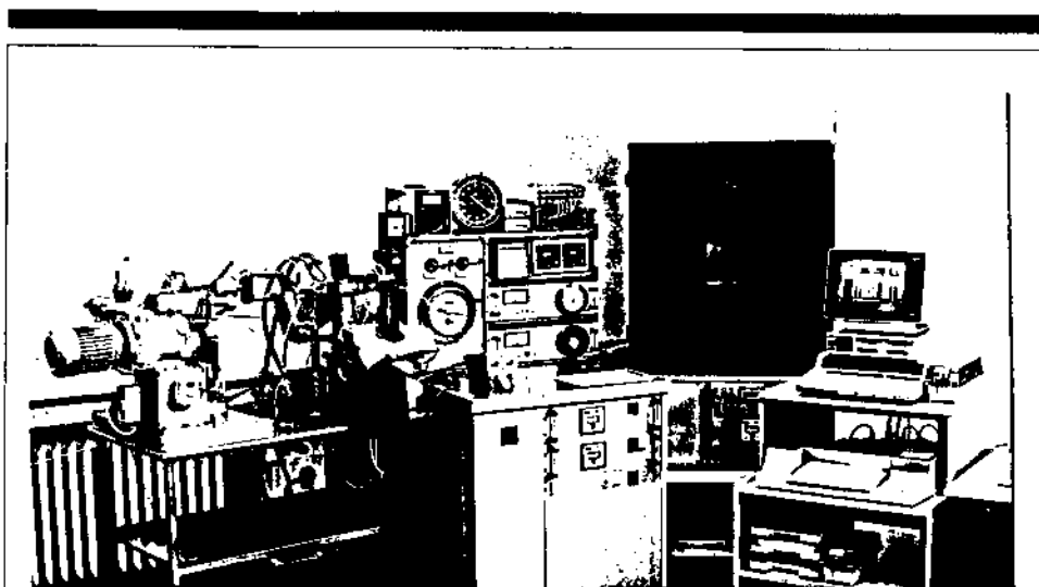
Figure 4 Test-rig with SCSR Mod. Auer SSR 120
